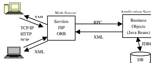
Figure 4: Sample 3-Tier Web Application Architecture
